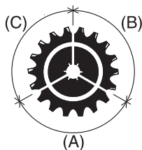
(A)Good (B)Abrasion teeth (C)Severe abrasion
